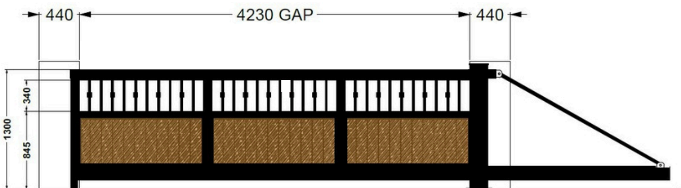
Drawing Provided for Installation Reference
